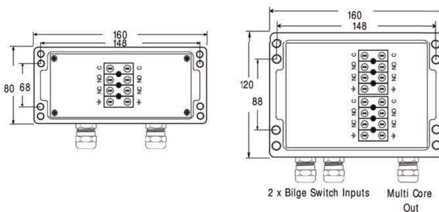
GA drawing (optional termination enclosure)
